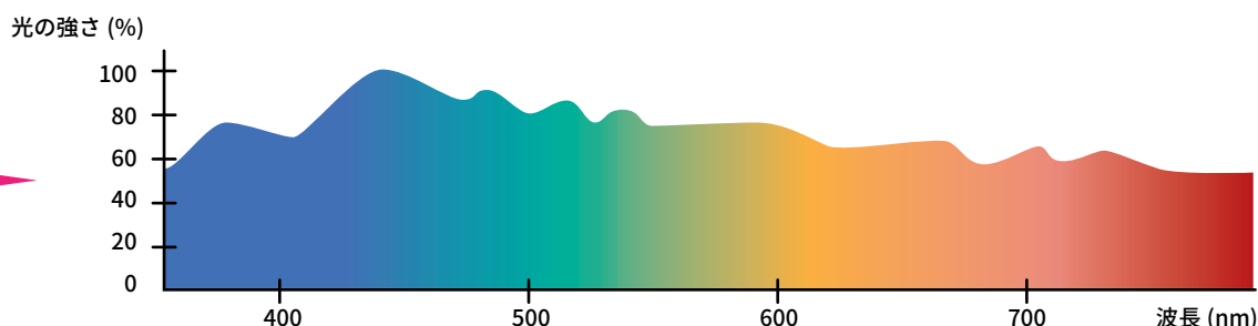
ECOLUX-H 分光分布
